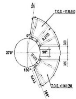
PLAN @ EL+1140.050 T.O.S.
